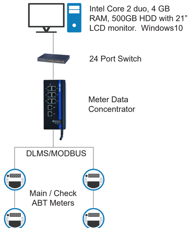
Figure 3 Configuration Diagram
